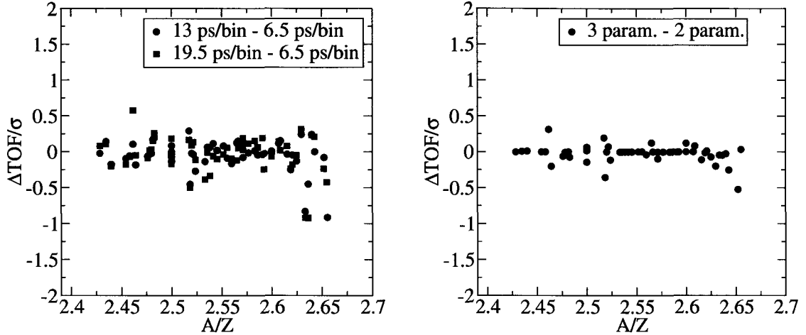
Figure 4.32: Sensitivity of the measured TOF centroid to the binning of the TOF (left) and the use of the standard deviation of the fit function as a free parameter (right). The change in the TOF shown in units of the statistical error in its determination ( \sigma ).
