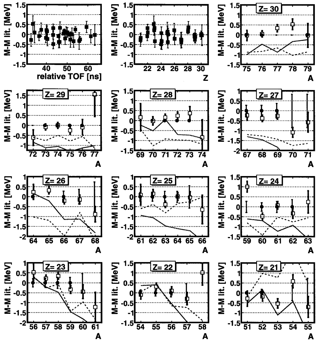
Figure 5.1: Mass results obtained in the present experiment. The first two graphs show the mass residuals for the fit of the calibration isotopes to the know masses as a function of their TOF ( A/Z ) and Z . These calibration isotopes are also indicated with black circles in the other graphs. The remaining graphs show the measured masses for each isotopic chain (red squares). The uncertainty in the literature data is shown as blue error bars around the zero axis, and extrapolated values from AME 2003 [4] are used to plot the residuals for the unknown masses (no error bars). In addition, the nuclear mass predicted by the FRDM (dashed green line) and the HFB-14 (solid green line) models is shown.
