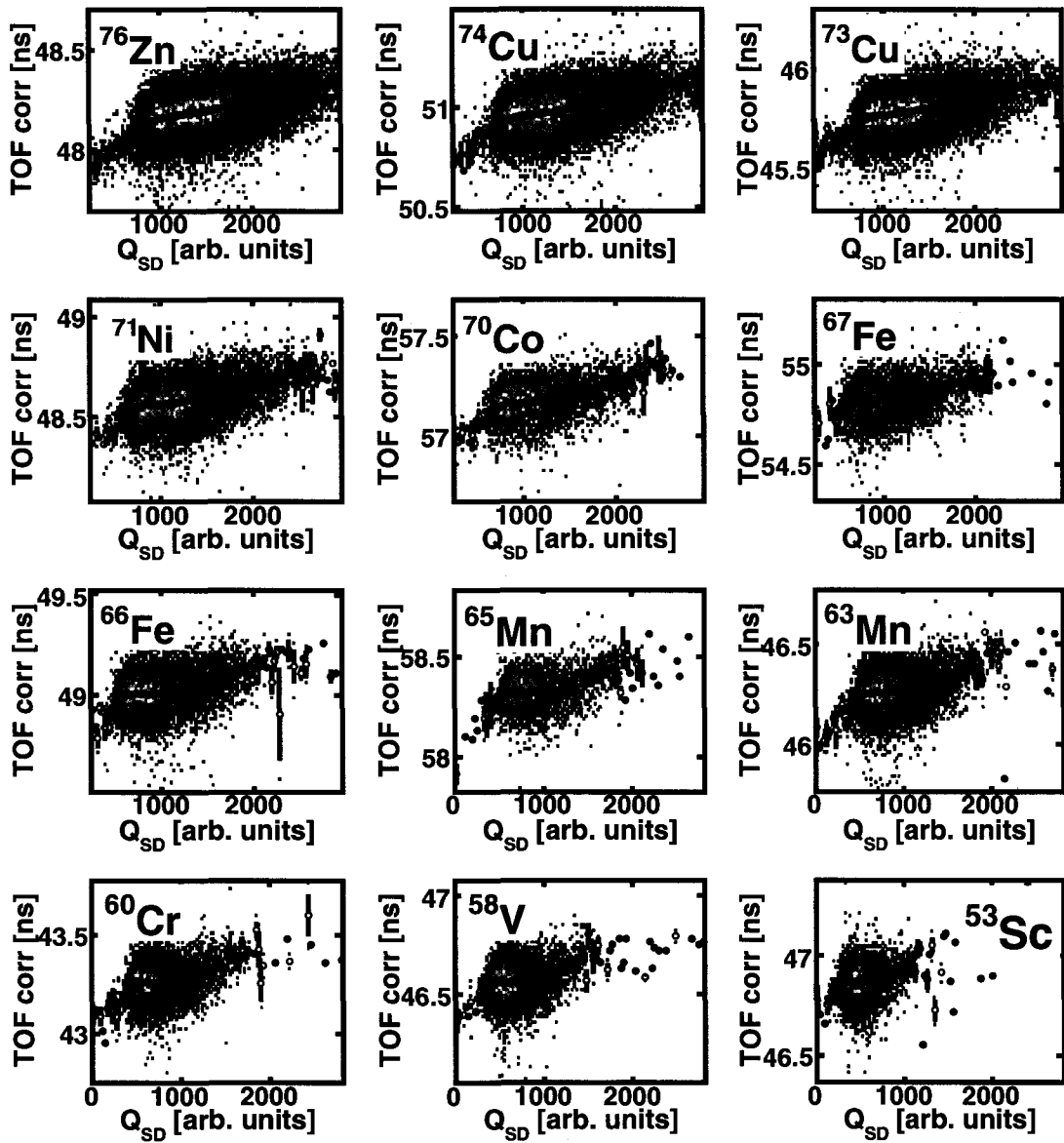
Figure 4.15: Momentum corrected TOF for selected isotopes in the beam as a function of the signal amplitude in the S800 Down photomultiplier tube of the timing detector. A profile histogram , which plots the average TOF value for each bin, is superimposed to the data and indicated with open circles.
