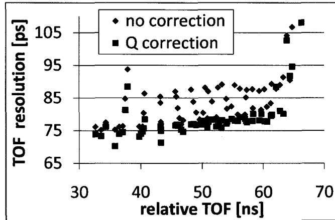
Figure 4.18: Width ( \sigma ) of the TOF distribution for events corrected only by their momentum ( TOF_{corr} , shown as light diamonds), and those with an additional correction for the signal amplitude in the PMTs following Equation 4.11 ( TOF_{corrQ} , shown as black squares).
