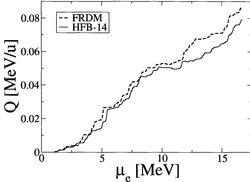
Figure 6.6: Energy released in the neutron star crust ( Q ) for calculations with an initial composition made up of the ashes of X-ray bursts [16]. The dashed line are the results for the FRDM mass model, and the solid line for the HFB one.
