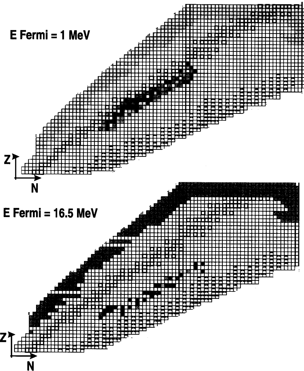
Figure 6.7: The top panel shows the composition of the C superburst ashes calculated by Schatz et al. [19] that are used as the initial condition for the crust calculation. This composition includes isotopes with a mass number up to A \sim 90 , but the most abundant species are in the range of 40 \leq A \leq 68 . The lower panel shows the neutron star composition at the end of the calculations ( \mu_e = 16.5 MeV) using the FRDM mass model. The color scale goes from red (more abundant isotope) to blue (less abundant). The bold squares indicate stable isotopes.
