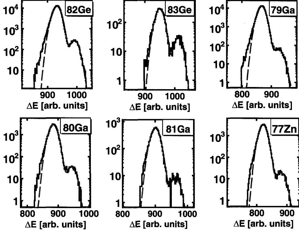
Figure 4.2: Energy loss spectra for a few ions and the overlapping charge states (higher \Delta E ), and a double gaussian fit to it.
