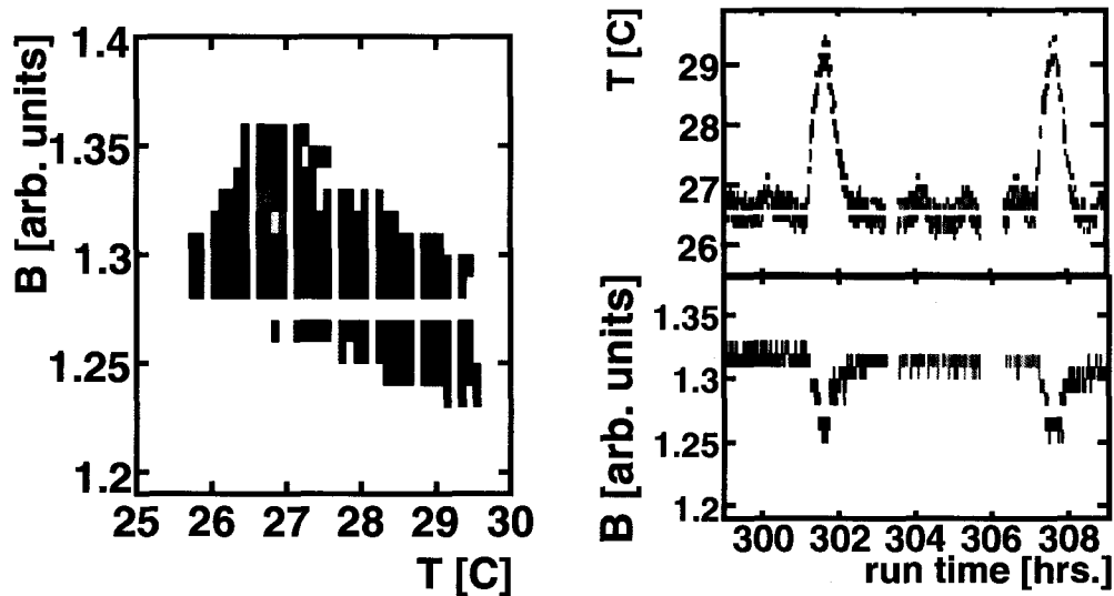
Figure 4.23: Correlation between temperature in S800 experimental vault and the magnetic field of the I265DS spectrometer dipole magnet. As explained in Section 3.3.1, the correlation results from the power supply for the dipole sharing the cooling water with the air conditioning unit in the vault. The figures on the right show data for only a fraction of the experiment.
