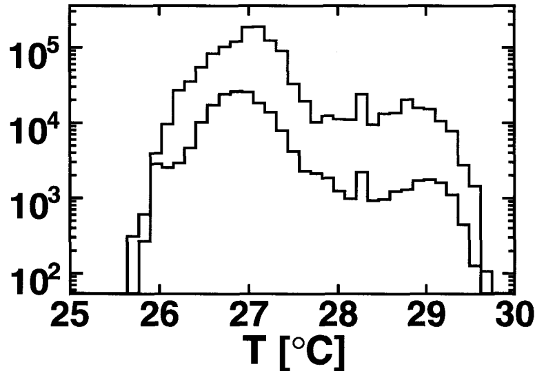
Figure 4.47: Temperature at the S800 experimental vaults for valid events during runs with the 94\text{ mg/cm}^2 (black) and the 47\text{ mg/cm}^2 (grey) Be production targets. As discussed in Section 3.1 different target thicknesses favors the transmission of fragments with different mass to charge ratio, so all isotopes in the beam should have similar temperature distributions in their events.
