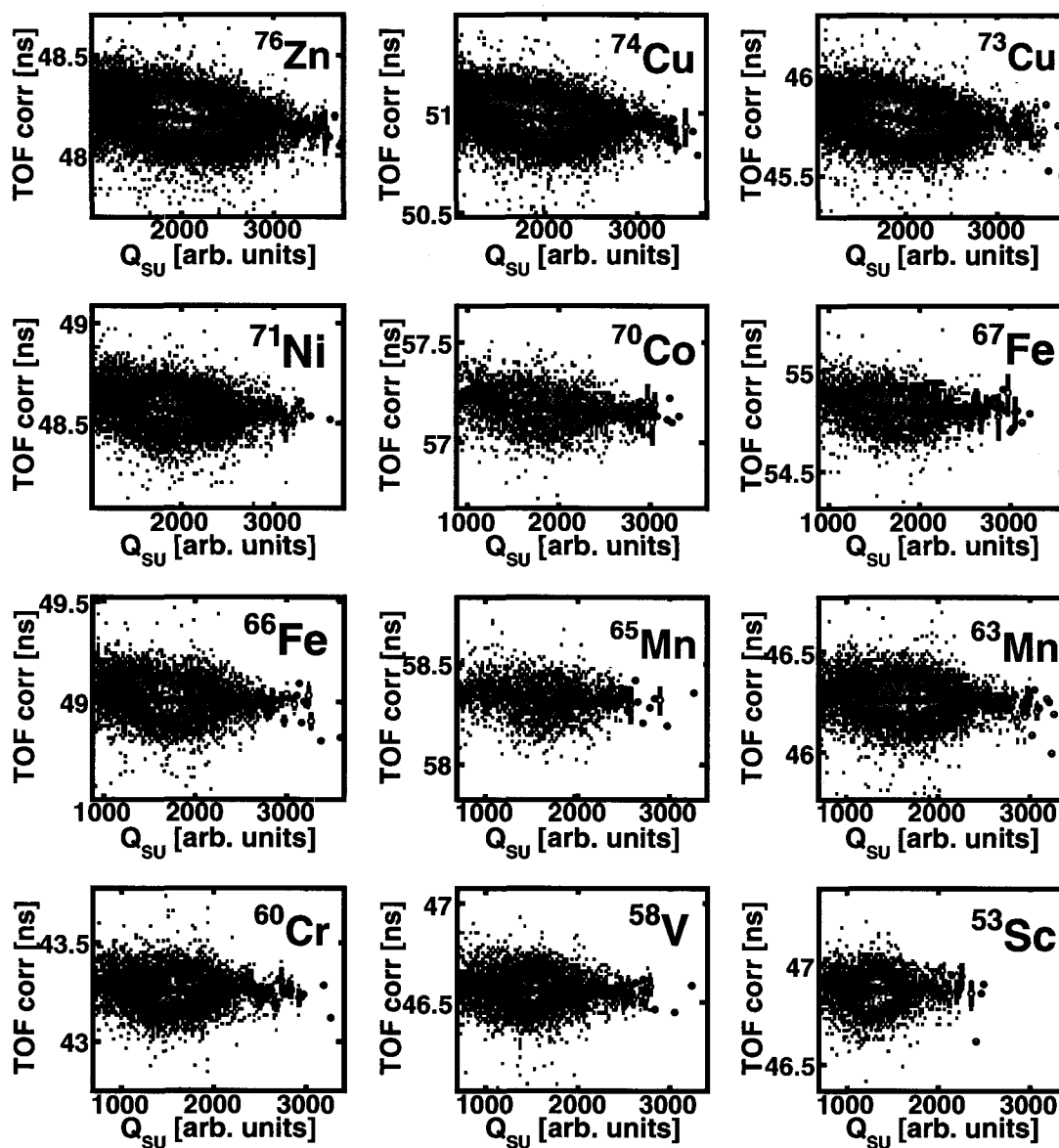
Figure 4.14: Momentum corrected TOF for selected isotopes in the beam as a function of the signal amplitude in the S800 Up photomultiplier tube of the timing detector. A profile histogram , which plots the average TOF value for each bin, is superimposed to the data and indicated with open circles.
