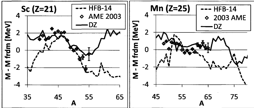
Figure 1.2: Mass results for the FRDM [21], HFB-14 [22], and Duflo-Zucker [29] mass models are compared to the data in the 2003 Atomic Mass Evaluation [4]. The nuclear masses are shown with respect to the FRDM model (zero). There is an increasing divergence of the mass predictions as one leaves the region of known data.
