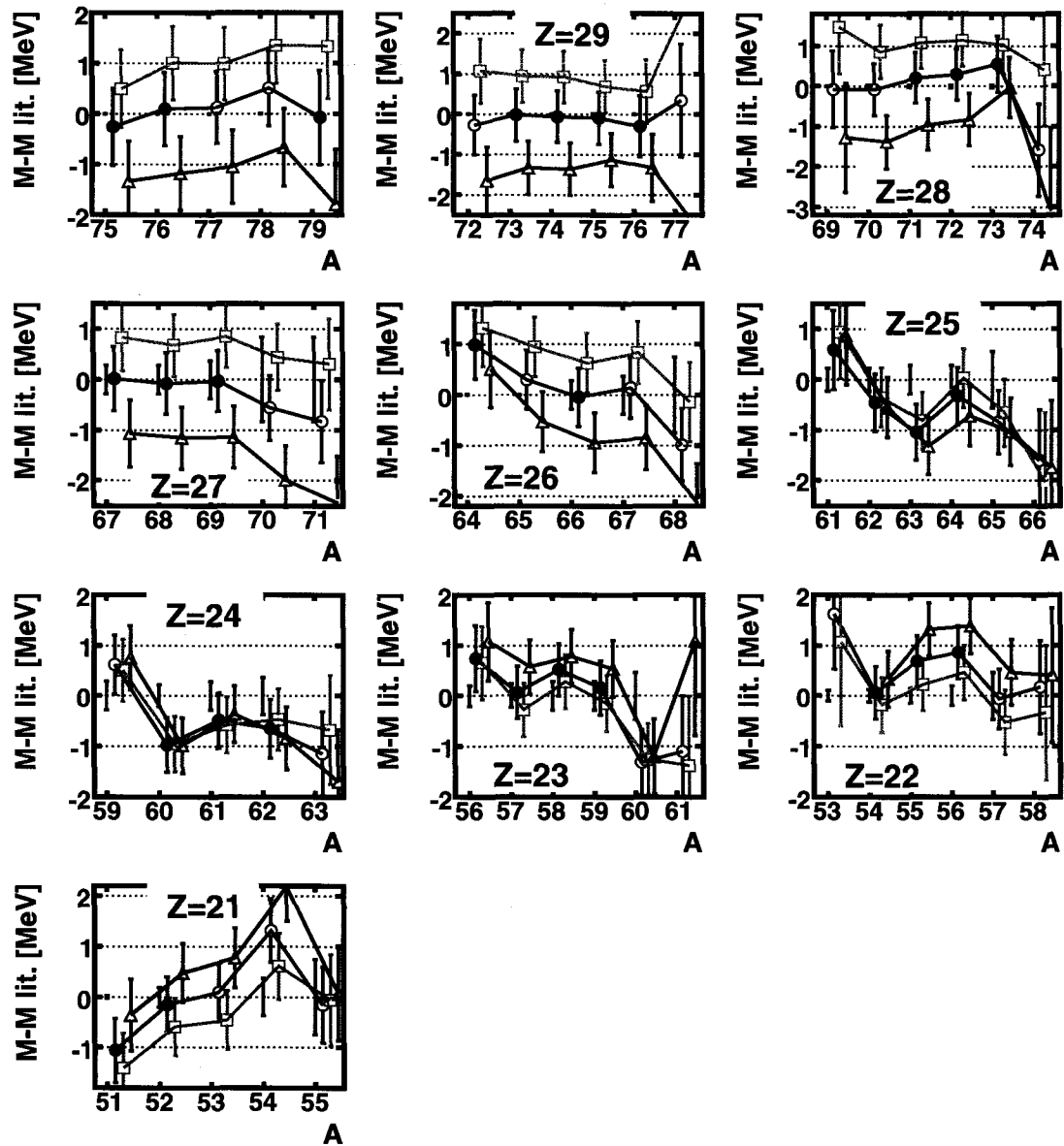
Figure 4.43: Sensitivity of the mass results to TOF correction by the a_{S800} angle. The mass calibration function was fitted to a set of TOF values corrected by a_{S800} angle, and the fit residuals are shown as red circles. The masses were then evaluated for sets of corrected TOF values that were determined with events with a positive (green squares) or negative (blue triangles) angle at the S800 focal plane. The masses for each isotopic chain are plotted with respect to the literature data (black error bars around the zero axis), using extrapolations in [4] when they are unknown.
