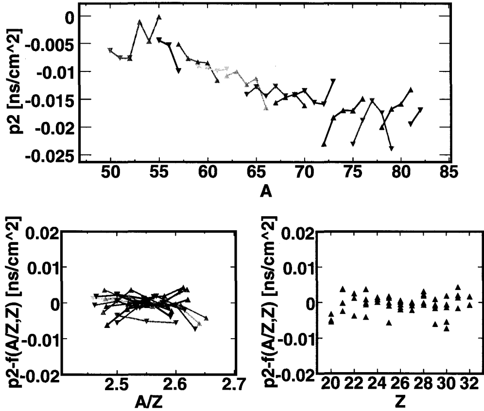
Figure 4.8: Fit for the quadratic term ( p_2 ) of a TOF momentum correction function quadratic in x_{\text{mcp}} . The top plot shows the quadratic term of fits of fits to the spectra of individual isotopes as a function of their mass ( A ). The lower plots show the residuals of the parameterization of these slopes by the equation 4.8. The weight given to each data point in the fit is the same as the one shown in Figure 4.7.
