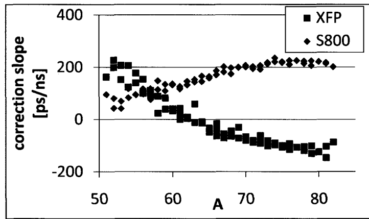
Figure 4.16: Results of the fits to the momentum corrected time of flight as a linear function of the time difference between the two PMT signals from each detector. The slope obtained for a linear fit of the TOF distribution of individual isotopes is shown as a function of their mass number A . A second order polynomial as a function of A was used to parameterize the slope of the correction function ( p_{\text{XFP}} and p_{\text{S800}} in Equation 4.11).
