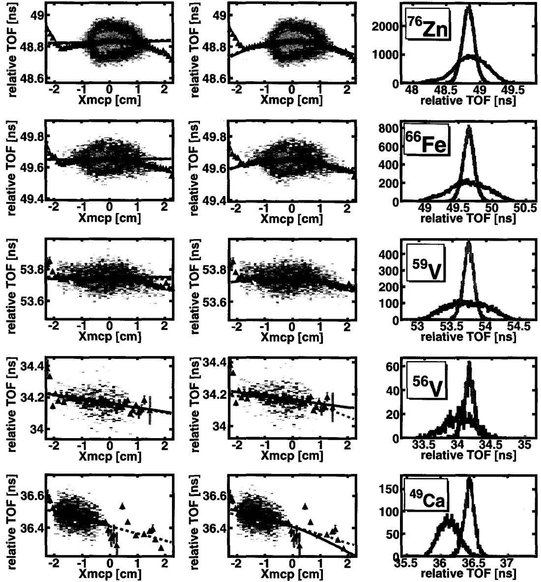
Figure 4.9: TOF vs x_{mcp} spectra for selected isotopes. The fits to each spectra using a linear (left graphs) and a quadratic (center graphs) are shown as black lines. In addition, the global parameterizations of the momentum corrections are shown as a dashed red line for the linear case, and as a dashed green line for the quadratic correction. For a better visualization of the results, a constant slope of 0.30 ns/cm was subtracted from all functions and from the data. The data is also shown as a Profile histogram (blue triangles), which plots the average content of each bin. The figures in the right column show the uncorrected TOF spectra (blue), as well as TOF_{corr} for the linear (red) and the quadratic (green) momentum corrections. Results for all isotopes in the secondary beam are shown in Appendix A.1.
