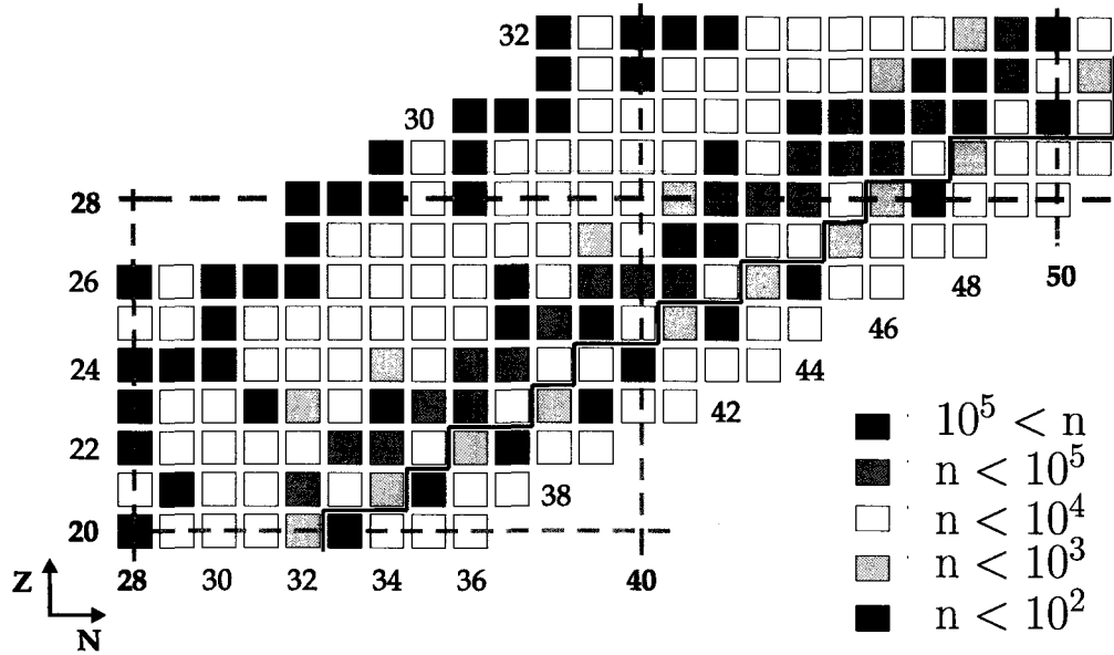
Figure 1.3: Region in the chart of the nuclides covered in the present time-of-flight experiment. The colored chart shows the number of events observed for each isotope in the secondary beam during the present time-of-flight experiment. Stable isotopes are indicated in black, and the solid black line indicates the limit of previously measured masses (Section 1.3).
