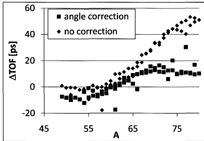
Figure 4.22: Difference in the TOF determined for events with a positive angle in the S800 focal plane versus those with negative angle. The difference is shown for the momentum corrected TOF_{corr} (light diamonds), and for the TOF_{corrA} of Equation 4.12, which is also corrected by its dependence on the PMT signal's amplitude and the S800 angle (black squares).
