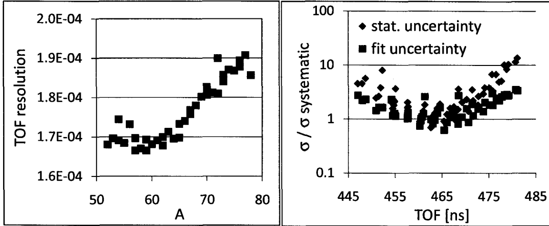
Figure 5.5: Relative time-of-flight resolution of the experimental setup (left), and contributions to the final mass error (right). The statistical uncertainty and the fit error (propagation of the uncertainty of fit parameters) are plotted relative to the systematic error obtained from the fit \chi^2 normalization (Section 4.5). The \sigma_{\text{sys}} was 3.4 keV/q, which corresponds to 85 keV for Mn isotopes ( Z=25 ).
