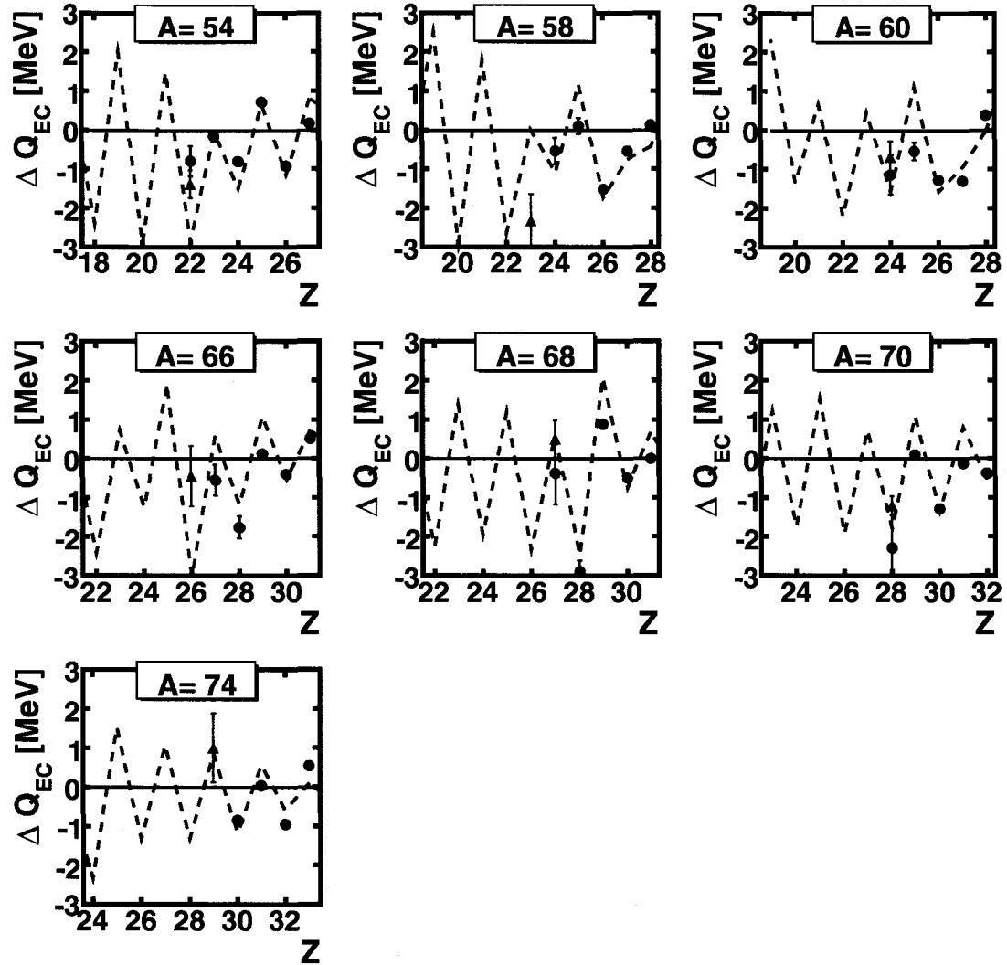
Figure 5.3: Electron capture Q -values for even A isobaric chains determined with the masses measured in this experiment. The Q -values are shown with respect to those calculated with the HFB-14 mass model ( \Delta Q_{EC} = Q_{EC}(i) - Q_{EC}(\text{HFB} - 14) ). The blue circles correspond to values calculated with the literature masses, the red triangles are calculated with the results of the present experiment. In addition, the dashed line shows the results for the FRDM model.
