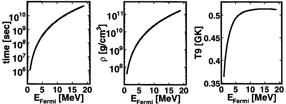
Figure 6.2: Thermodynamic trajectories for the neutron star crust used by the reaction network solver [74].
