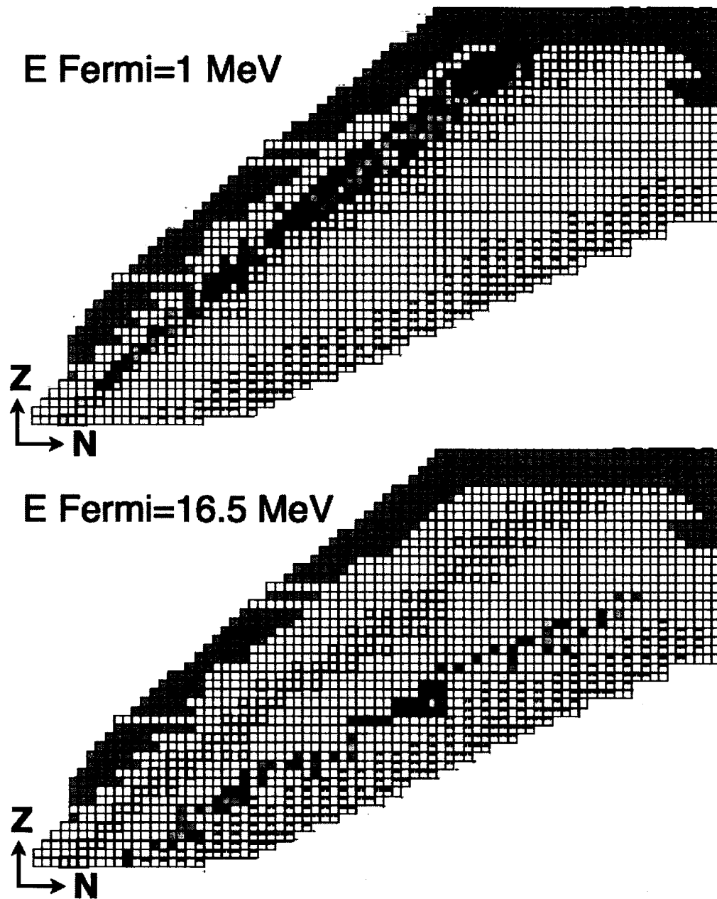
Figure 6.5: The top panel shows the composition of the X-ray burst ashes calculated by Schatz et al. [16] that are used as the initial condition for the crust calculation. This composition includes isotopes with a mass number up to A \sim 110 . The lower panel shows the neutron star composition at the end of the calculations ( \mu_e = 16.5 MeV) using the HFB-14 mass model. The color scale goes from red (more abundant isotope) to blue (less abundant). The bold squares indicate stable isotopes.
