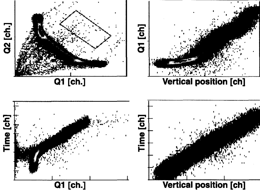
Figure 2.4: The upper panels show the correlations between the signal amplitude (Q) recorded in each PMT, and between the vertical position in the plastic scintillator and the signal amplitude in the PMT1. The spectra in the lower panels show the time difference between the signals from the photomultiplier tube PMT1 (start) and PMT2 (stop) as a function of the signal amplitude in one PMT and the vertical position in the plastic scintillator. They correspond to a run with a bias voltage of -1.6 kV of the PMTs. In this run the width of the time spectra obtained using a linear correction for the vertical position is 26.5 ps (Figure 2.6).
