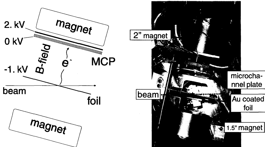
Figure 3.12: Diagram of microchannel plate (MCP) detectors used for position measurement at the S800 dispersive plane [63]. The picture shows the MCP1 detector arranged in a close configuration to increase the magnetic field at the channel plate; the x_{\text{mcp}} position measured with this detector was used to determine the momentum of the beam particles.
