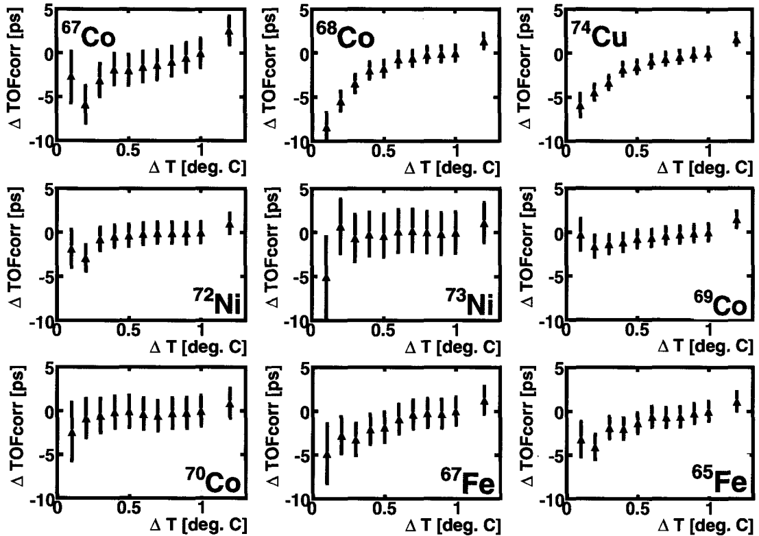
Figure 4.25: Sensitivity of the measured TOF for cuts in the S800 vault temperature spectra. The momentum corrected TOF was determined for events when the measured temperature was in the range of 27^{\circ}\text{C} \pm \Delta T , and compared to the TOF determined for 26^{\circ}\text{C} \leq T \leq 28^{\circ}\text{C} .
