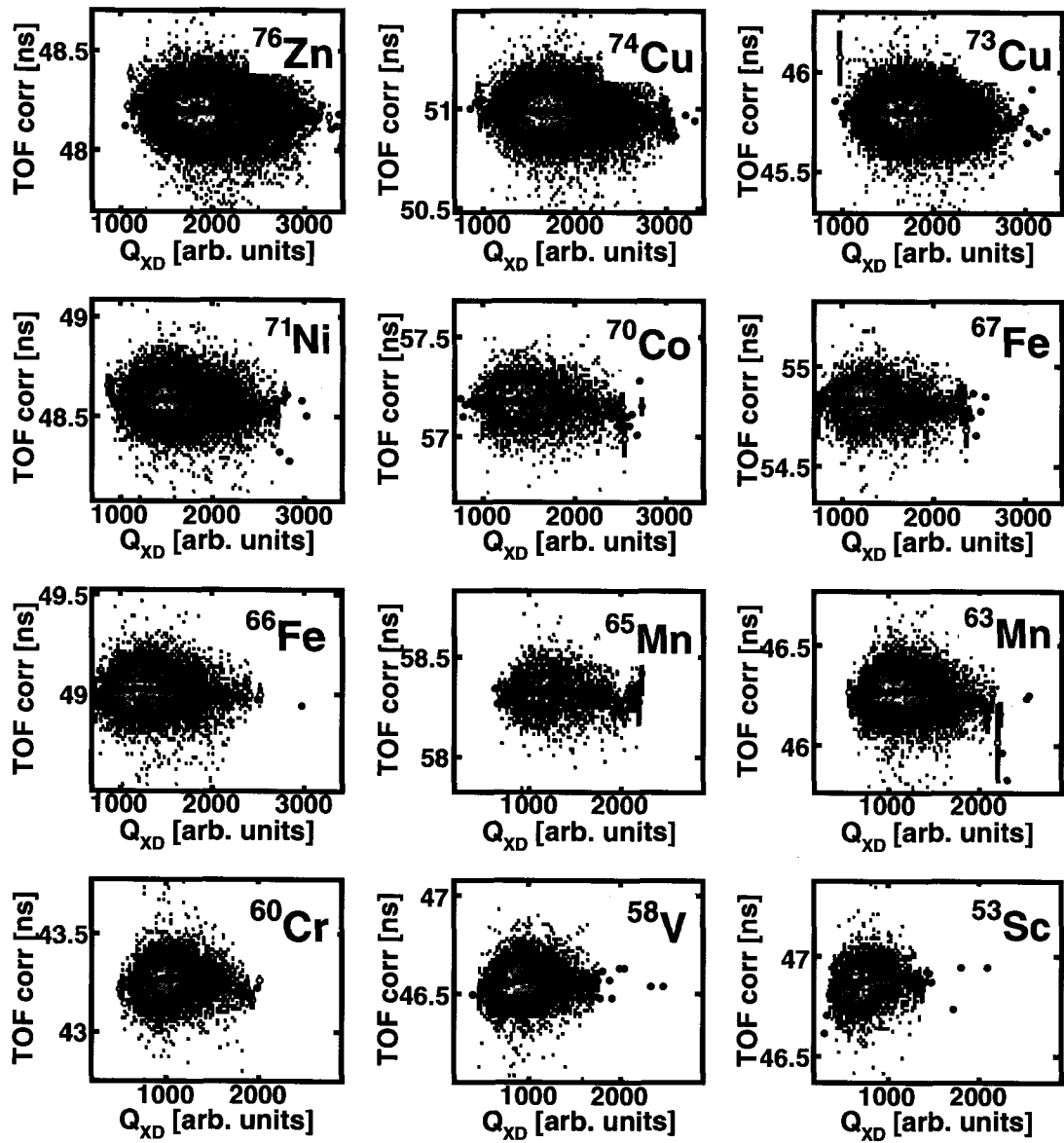
Figure 4.13: Momentum corrected TOF for selected isotopes in the beam as a function of the signal amplitude in the XFP Down photomultiplier tube of the timing detector. A profile histogram , which plots the average TOF value for each bin, is superimposed to the data and indicated with open circles.
