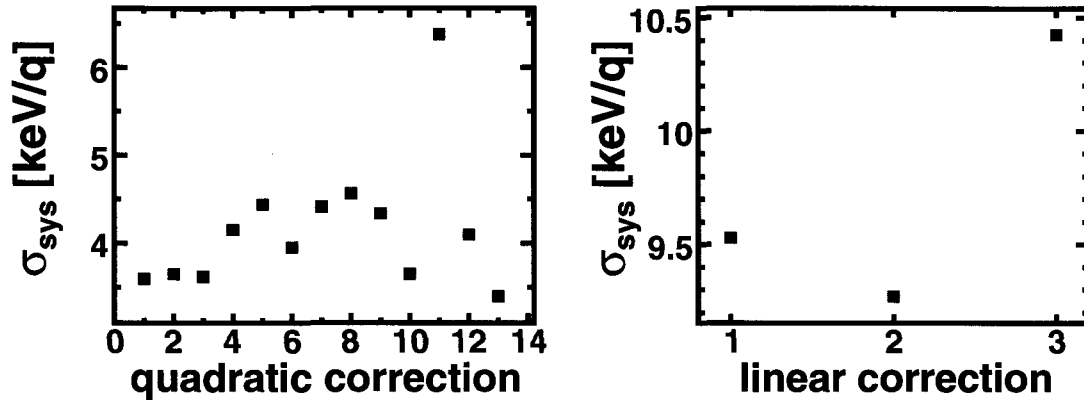
Figure 4.36: Estimate of the fit systematic error ( \sigma_{\text{sys}} ) for arbitrary variations in the parameters of the quadratic (left) and linear (right) B\rho correction functions. Fit 1 corresponds to the data evaluated using the original parameters for the correction functions. For the quadratic momentum case (left graph), the fits 2 through 9 are all possible combinations when the coefficients are increased or decreased by 1.5% (for 2 and 3 only the quadratic coefficient is changed, and for 4 to 9 the linear slope is also changed). The remaining four fits are obtained when increasing or decreasing one of the coefficients by 3% (10 and 11 for the slope, and 12 and 13 for the quadratic term). For the linear B\rho correction, fit 2 corresponds to TOF data corrected with a slope that was increased by 1.5%, and decreased by the same amount for fit 3.
