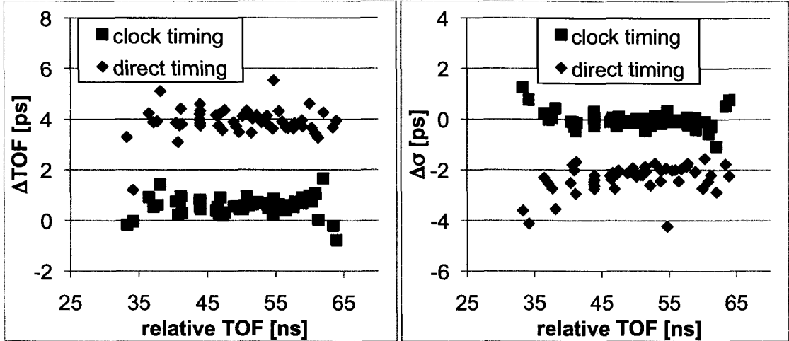
Figure 4.30: The figure shows the change in the measured TOF ( \Delta TOF ), and in the width of the TOF spectra ( \Delta\sigma ), when using a cut to reject events with a glitch in the electronic modules. The cut produces a small improvement in the resolution for the direct time measurement, and shifts the measured TOF of all ions. The clock is also shown to be less sensitive to this effect, since it does not use the Scintillator Fan S3 module (Figure 4.28).
