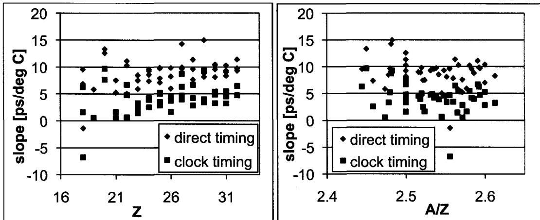
Figure 4.26: Slope resulting from a linear fit to the dependence of TOF_{\text{corr}} on the temperature in the S800 vault for the different isotopes in the secondary beam. Note that the correlation between TOF and temperature is always larger for the TOF determined from the direct measurement between the timing signals ( TOF_1 ) than for the measurement with respect to a clock ( TOF_{\text{clk}} ).
