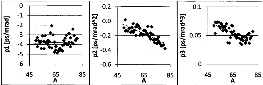
Figure 4.21: Results for the fit of the time of flight correction by the a_{S800} angle. The parameters of a cubic polynomial (Equation 4.12) fit to the TOF distribution of individual isotopes are shown as a function of their mass number A . A linear parameterization of these fit results as a function of A was used for the calculation of TOF_{corrA} .
