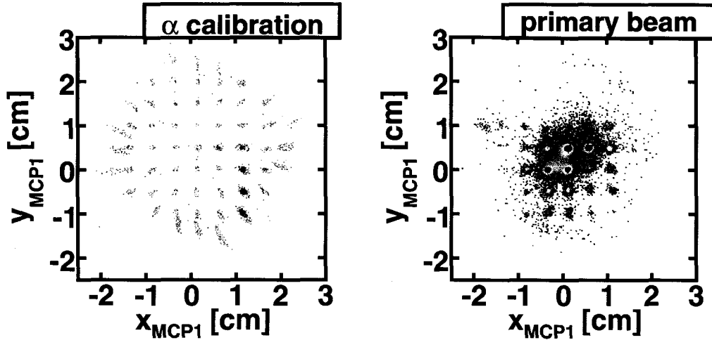
Figure 3.14: Mask position calibration of the MCP detector. A calibration function [63] for the raw detector spectra was obtained with a calibration done with an alpha source (left). A mask run was performed with a degraded primary beam ( ^{86}\text{Kr} ) to check the calibration for the position measured with heavy ions (right).
