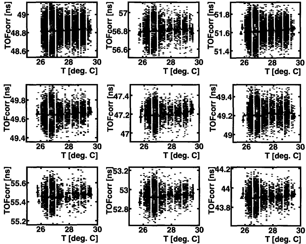
Figure 4.24: For a few isotopes the momentum corrected TOF_{corr} is shown as a function of the temperature in the S800 experimental vault. The observed correlation is of the order of 10 ps/°C for the direct TOF measurement, and about 5 ps/°C for the TOF measured with respect to a clock.
