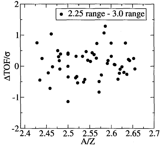
Figure 4.33: Sensitivity of the measured TOF centroid to the range of the function used to fit its spectra. A Gaussian function was iteratively fit to the TOF spectra using only events within a given number of standard deviations from the centroid. The change in the TOF centroid obtained using 3 or 2.25 standard deviations as the fit range is shown in units of the statistical error in TOF centroid determination ( \sigma ).
