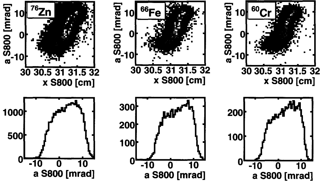
Figure 4.20: The upper figures show the correlation between the angle and position at the location of the S800 timing detector (S800 focal plane) for a few isotopes in the beam. The correlation between both variables shows that the beam was focused a few centimeters after the detector. The angular distribution is very similar for all species in the beam.
