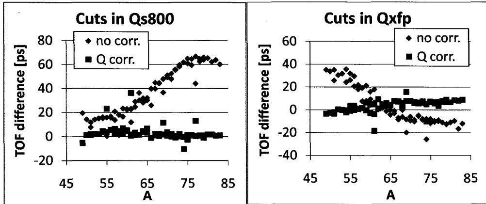
Figure 4.17: TOF determined for events with different amplitude in the PMT signals. The left (right) figure shows the difference in the determined TOF for events with a large signal in Q_{S800down} ( Q_{XFPdown} ) versus the TOF determined from the events with a low amplitude signal in that detector. The difference is shown for a TOF that was only corrected by the particles momentum ( TOF_{corr} , shown as light diamonds), and also for data that was also corrected by their t_{SUSD} and t_{XUXD} following equation 4.11 ( TOF_{corrA} , shown as black squares).
