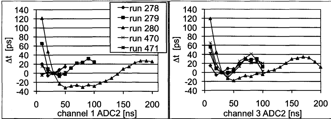
Figure 3.7: Results of the time calibrations for channel 1 of ADC2 (left) and channel 3 of ADC2 (right). The figures show the residuals ( \Delta t ) from a linear calibration function for runs with different settings for the TAC range: 50 ns in run 278, 100 ns in run 279, 200 ns in run 280, and range used in the experiment for runs 470 and 471 (50 ns for channel 1 and 100 ns for channel 3).
