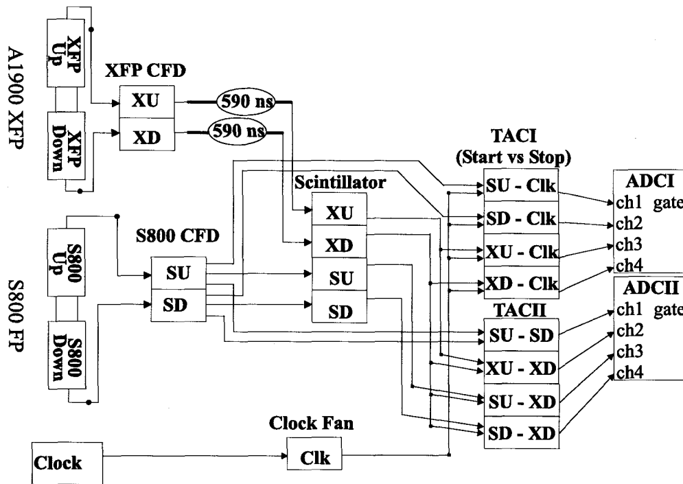
Figure 4.28: Electronics diagram for the timing subsystem.
