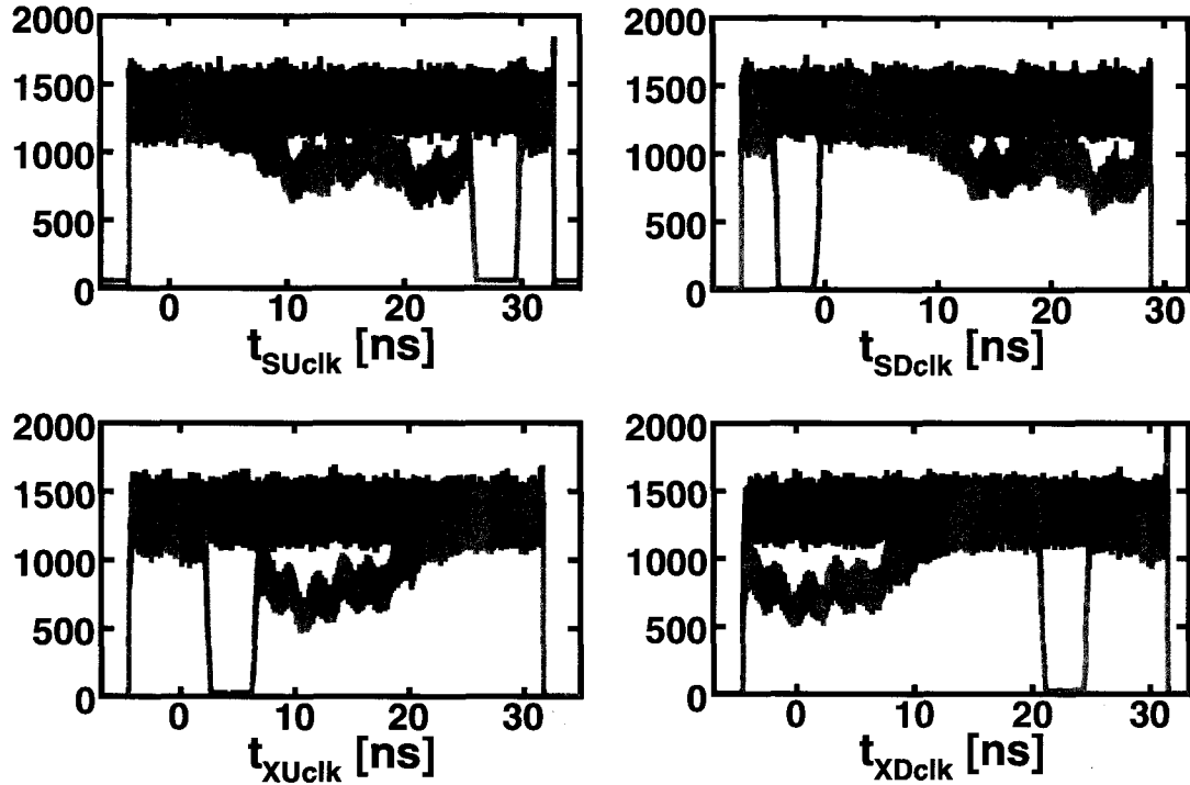
Figure 3.10: ADC spectra for the four channels that time each PMT signal with respect to the clock. All events for isotopes with Z \gtrsim 15 are shown. The grey spectra correspond to events where a valid signal is required in all four ADC channels. Because the signals of the two PMTs in each timing scintillator are correlated in time, the blind region of the TAC range (short time from start to stop) is observed in the spectra from the signal of the companion PMT. The spectra also present a large channel to channel variation that is an artifact of the bin width used.
