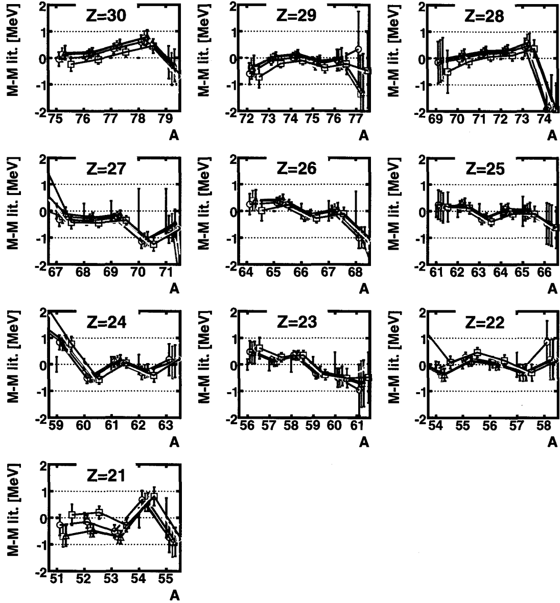
Figure 4.38: Evaluation of the mass calibration function using a sets of TOF values determined with arbitrary parameters of a quadratic B\rho correction. The parameters of the mass calibration function were fitted to TOF data obtained with the B\rho correction of Section 4.2 (red circles). The other series correspond to data when the slope ( p1 ) and the curvature ( p2 ) of the B\rho correction were changed by: \delta p1 = -1.5\% and \delta p2 = -1.5\% (green squares), \delta p1 = -1.5\% and \delta p2 = 1.5\% (blue triangles), \delta p1 = 1.5\% and \delta p2 = -1.5\% (yellow diamonds), \delta p1 = 1.5\% and \delta p2 = 1.5\% (magenta squares). The masses are shown with respect to the literature data, and the extrapolations in [4] are used when the mass is not known. The uncertainty in the literature values is shown as black lines around the zero axis.
