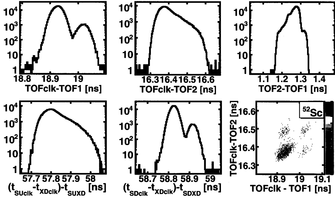
Figure 4.29: Comparison of semi-independent time-of-flight measurements (equation 4.13). About 10 % of the events are shifted by 90 ps by a glitch that was traced to the electronic logic modules that multiply the signals from the S800 timing detectors. The two dimensional spectra only shows events of one isotope ( ^{52}\text{Sc} ).
