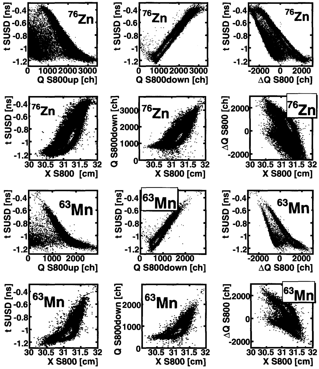
Figure 4.10: Correlations between signal amplitude from the S800 PMTs with the timing between both PMTs and the x_{\text{S800}} position for ^{76}\text{Zn} ( Z=30 ) and ^{63}\text{Mn} ( Z=25 ) events. The difference between both signal amplitudes is also shown ( \Delta Q_{\text{S800}} = Q_{\text{S800up}} - Q_{\text{S800down}} ).
