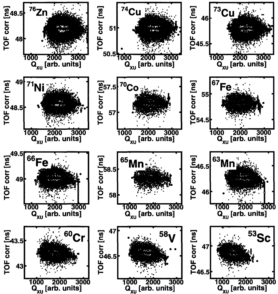
Figure 4.12: Momentum corrected TOF for selected isotopes in the beam as a function of the signal amplitude in the XFP Up photomultiplier tube of the timing detector. A profile histogram , which plots the average TOF value for each bin, is superimposed to the data and indicated with open circles.
